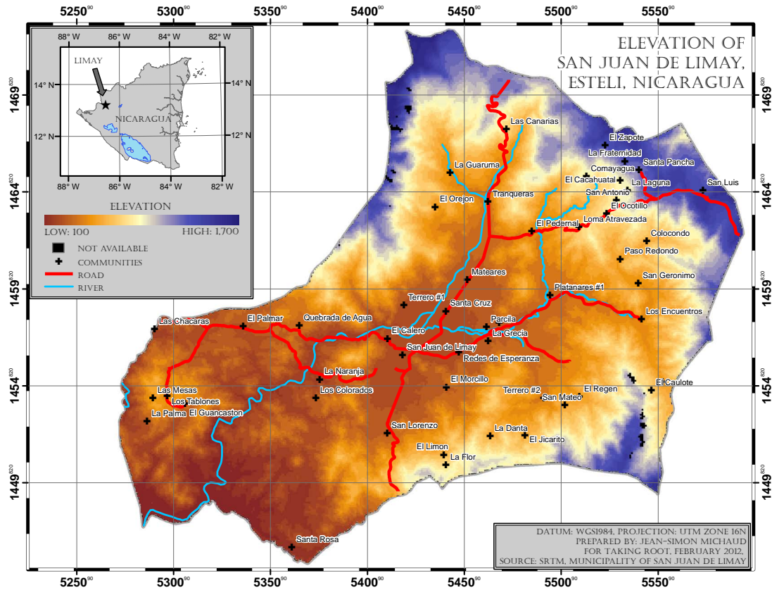
Figure 2 - Elevation map of San Juan de Limay.
